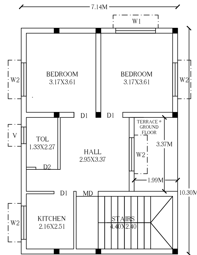
TYPICAL GROUND, FIRST & SECOND FLOOR PLAN
